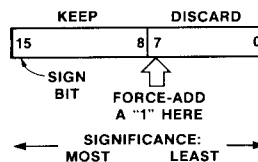
Figure 7. Unsigned Rounding
