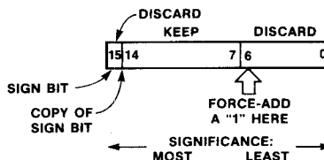
Figure 8. Signed Rounding
