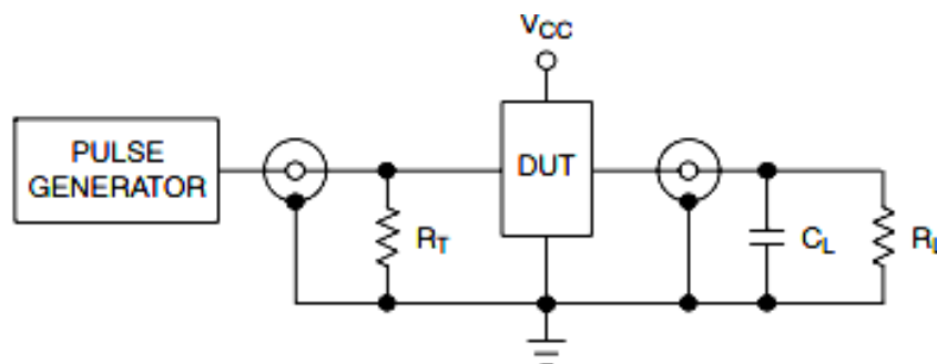
Figure4. Test Circuit
