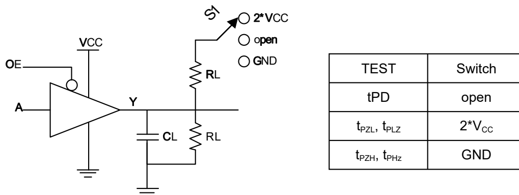
Figure5. Output enable/disable Time Test Circuit
