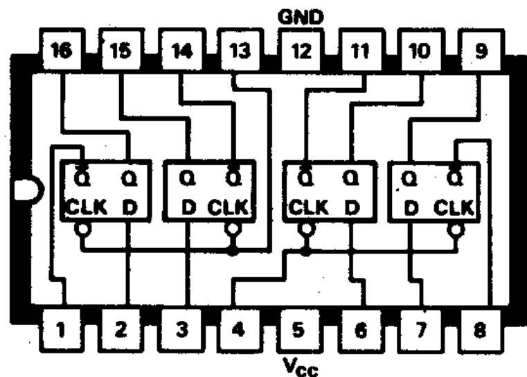
B56 SN7475N Quad bistable latch
