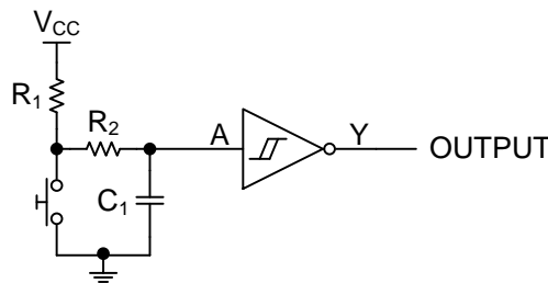
Figure 7. Push Button Debounce Circuit Schematic
