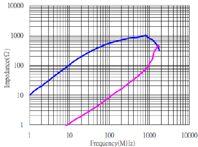
SMW4532B601G
