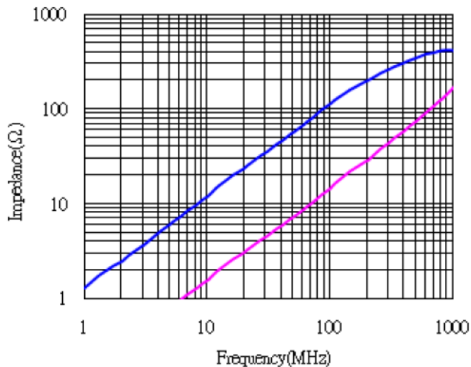
SMW4532B121G
