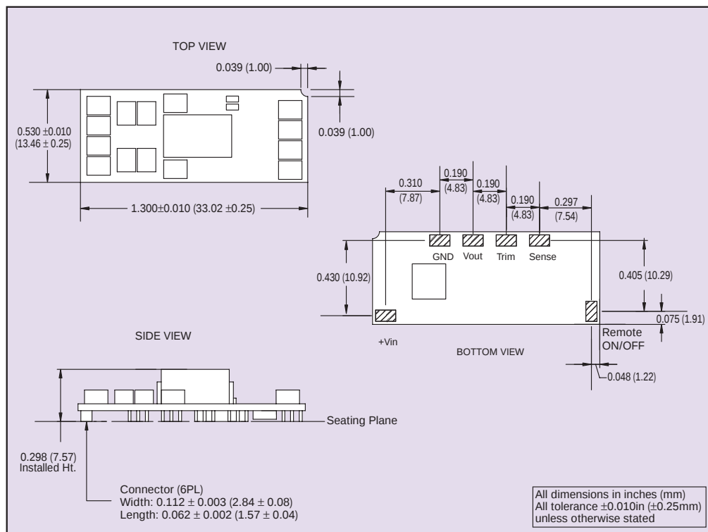
Figure 5 - Mechanical Drawing
