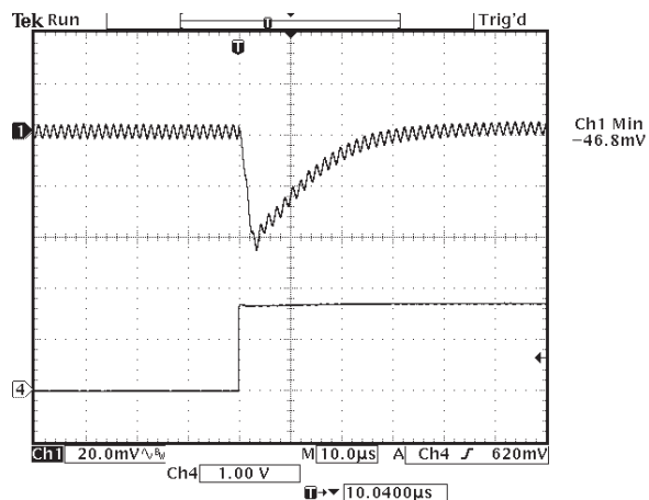
Figure 3 - Typical Transient Response, (Vin = 12 V, Output Current = 1.2 V), 7.5 A Load Step Change; Slew Rate = 200 A/μs Channel 1: Voltage Deviation = 46.8 mV; Recovery Time = 10 μs
