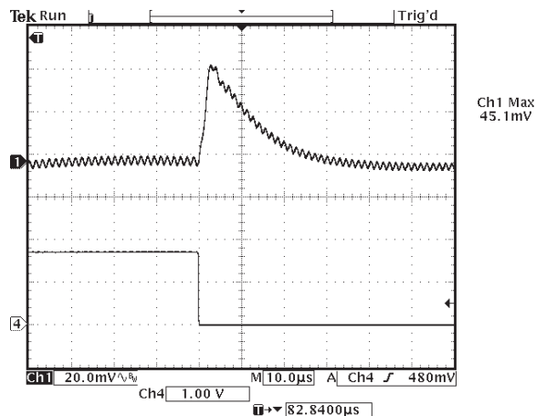
Figure 2 - Typical Transient Response, (Vin = 12 V, Output Current = 1.2 V), 7.5 A Load Step Change; Slew Rate = 200 A/μs Channel 1: Voltage Deviation = 45 mV; Recovery Time = 10 μs
