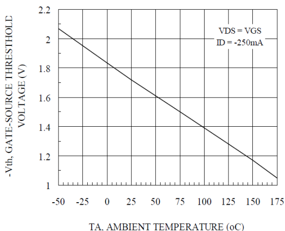
Figure 9. Vth Gate to Source Voltage Vs Temperature
