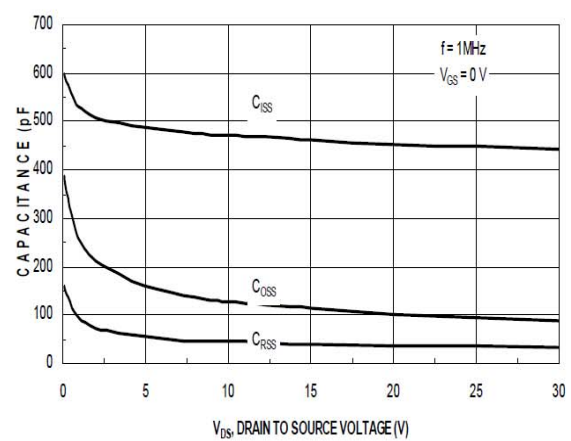
Figure 4. Capacitance Characteristics
