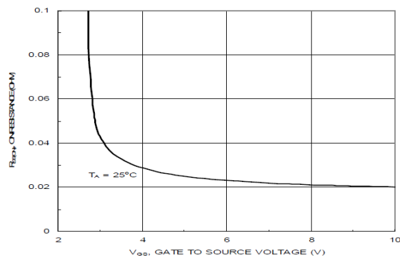
Figure 8. On-Resistance with Gate to Source Voltage
