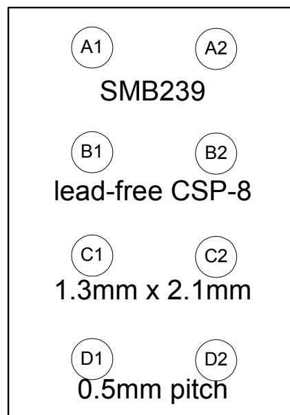
Bottom View (Balls facing up)
