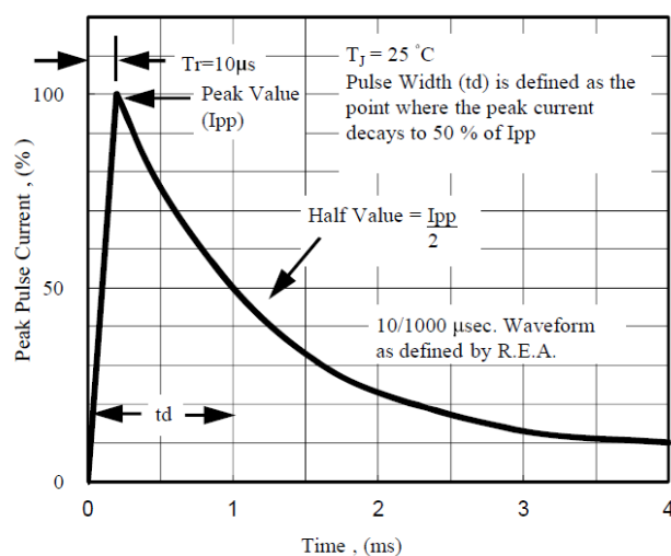
Fig. 5 - Pulse Waveform
