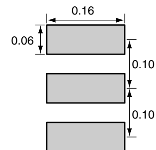
RECOMMENDED FOOTPRINT
