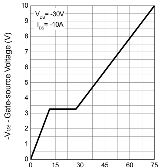
Gate Charge
