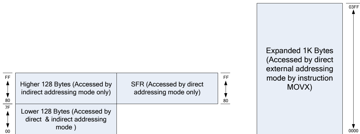
Fig. 3-3: RAM architecture
