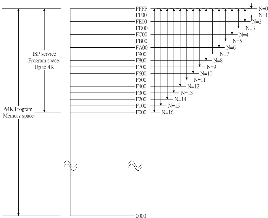
Fig. 3-1: SM59R16A5 programmable Flash
