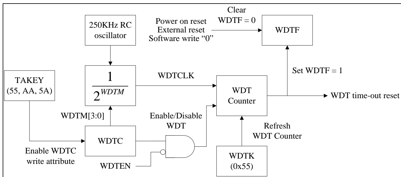
Fig. 10-1: Watchdog timer block diagram
