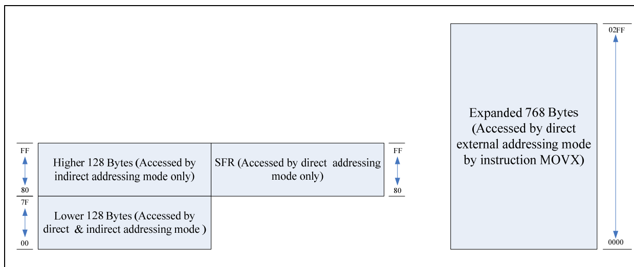
Fig. 3-2 : RAM architecture
