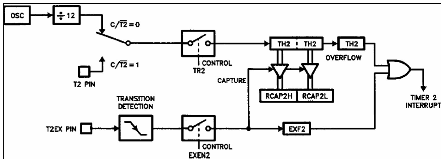
Figure 7-1 : Timer 2 in capture mode
