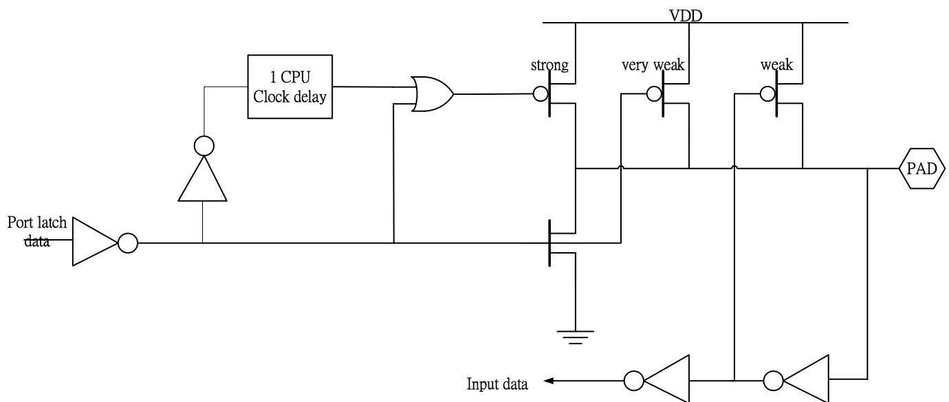
Fig. 1-1 : IO pad structure
