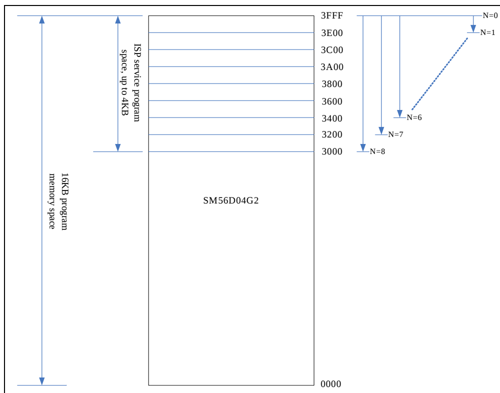
Fig 3-1 : Flash segmentation for ISP
