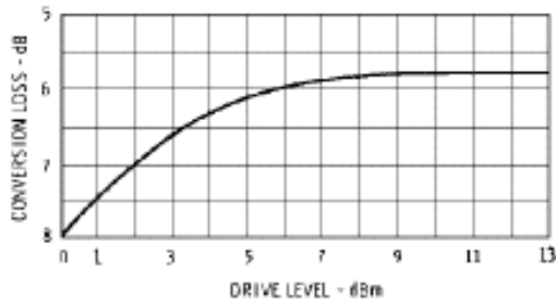
Conversion Loss
