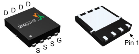
DFN5x6-8
