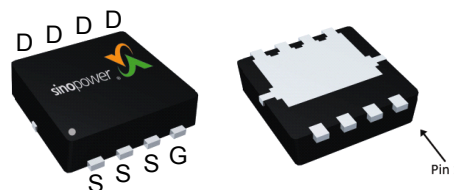
DFN3.3x3.3A-8_EP
