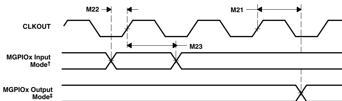
Figure 5–21. McBSP General-Purpose I/O Timings
