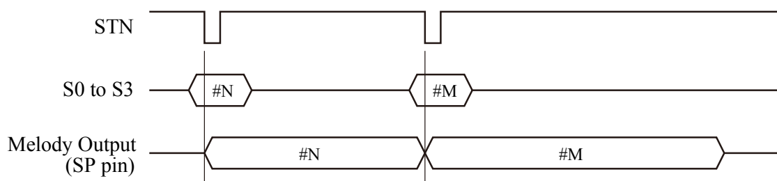
Figure 5. One-shot mode
