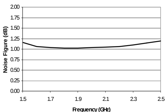
Noise Figure
