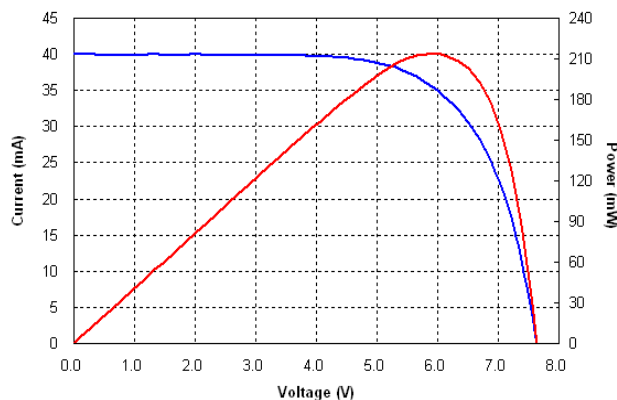
Current-Voltage Characteristics
