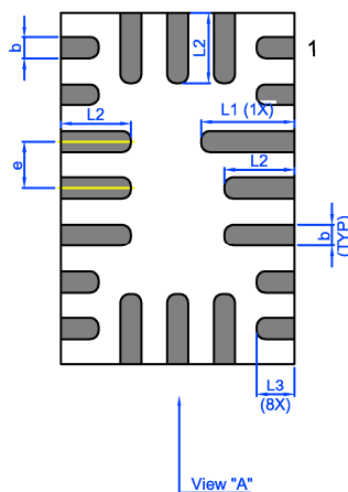
BOTTOM VIEW
