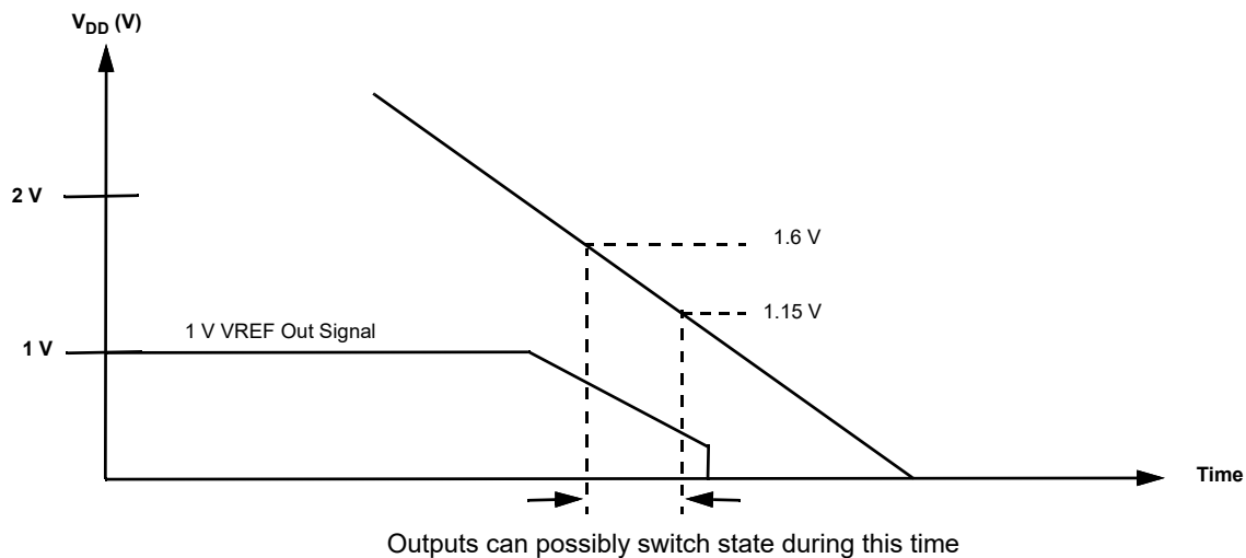
Figure 44. Power Down
