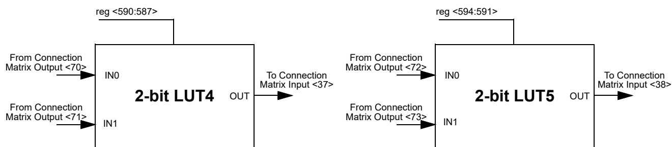
Figure 7. 2-bit LUTs
