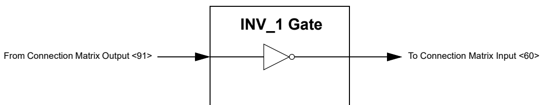
Figure 35. INV_1 Gate
