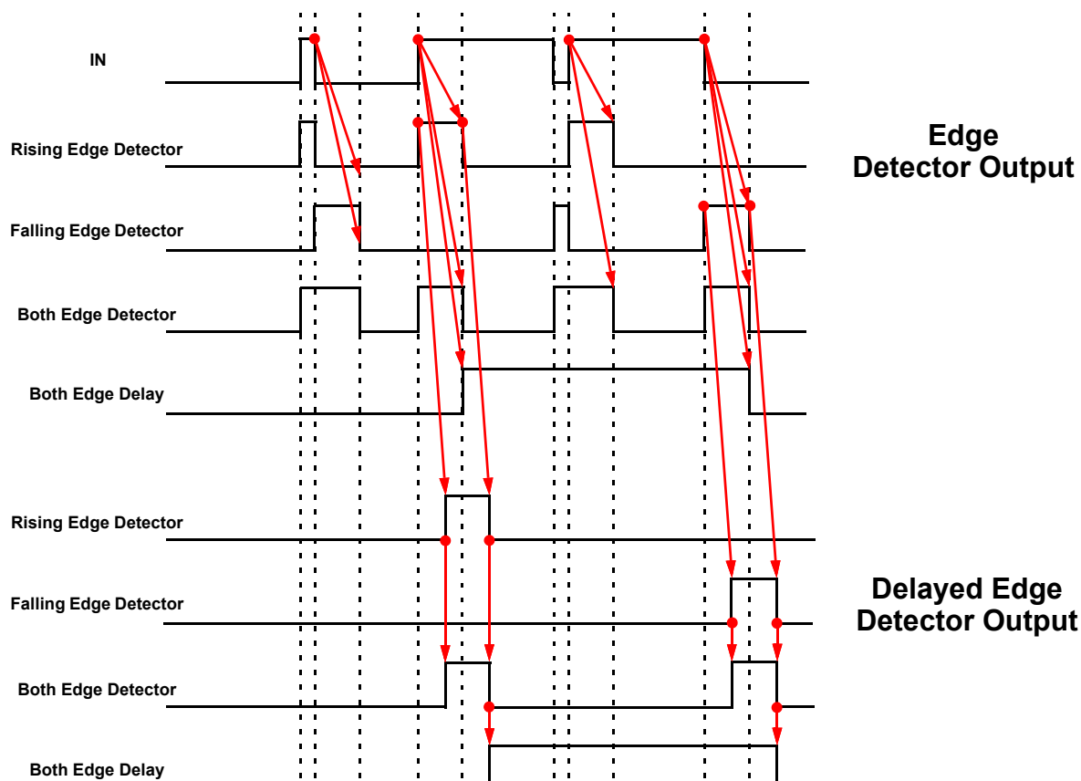
Figure 33. Glitch Filtering for Edge Detector Output
