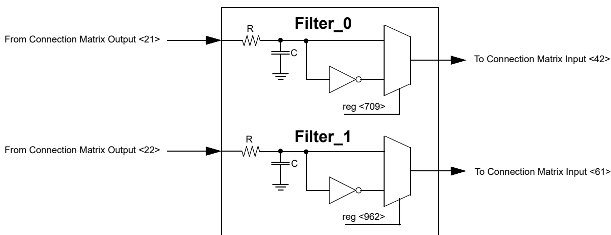
Figure 36. Deglitch Filter
