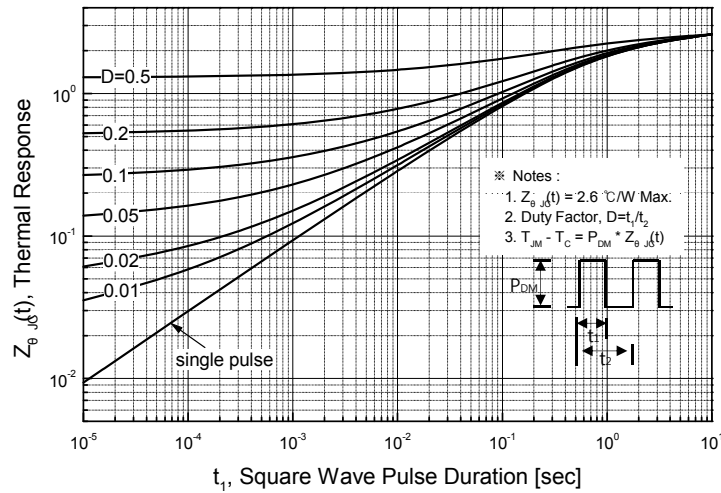
Figure 11-2. Transient Thermal Response Curve for SLF6N70U
