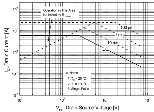
Figure 9-2. Maximum Safe Operating Area for SLF6N70U
