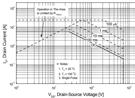
Figure 9-1. Maximum Safe Operating Area for SLP6N70U
