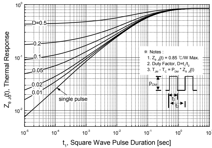
Figure 11-1. Transient Thermal Response Curve for SLP6N70U
