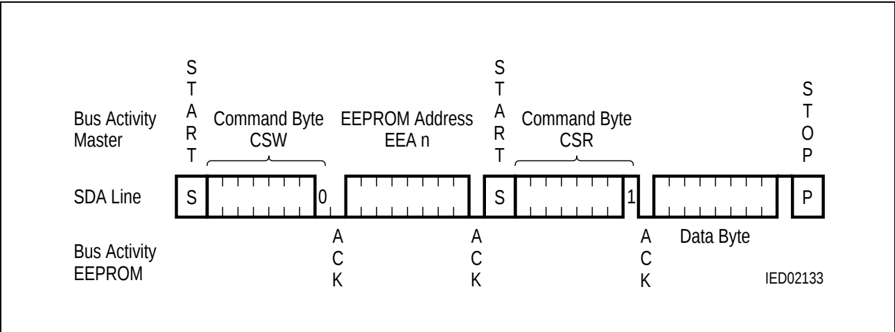
Figure 11 Random Read
