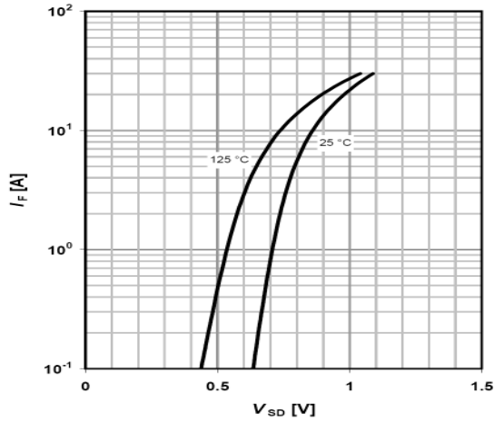
Figure 7: Body-Diode Characteristics
