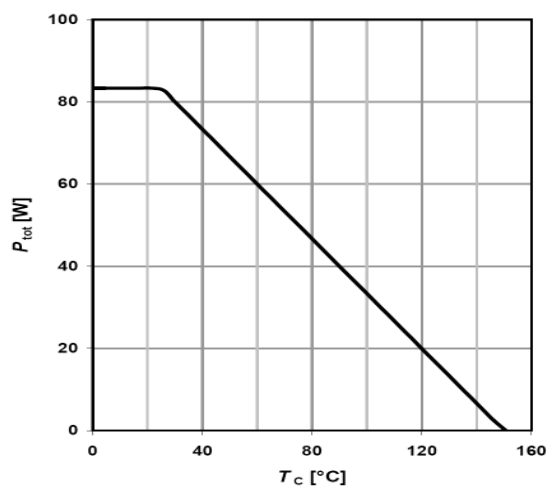
Figure 3: Power Dissipation
