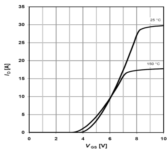
Figure 14: Typical transfer characteristics
