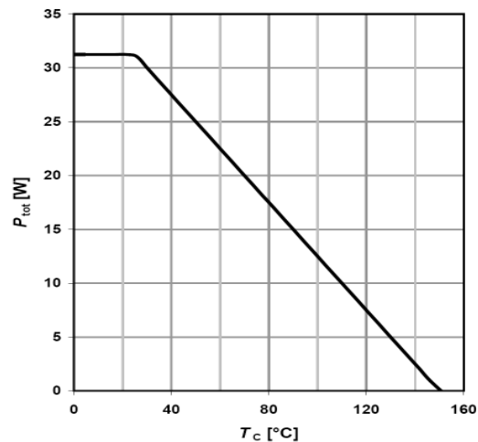
Figure 4 : Power dissipation
