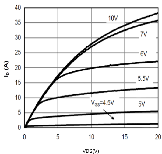
Figure 1: On-Region Characteristics@25°C
