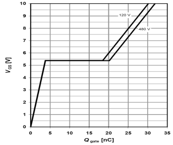
Figure 8: Gate-Charge Characteristics
