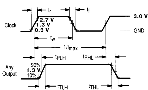
Figure 1. Switching Waveforms
