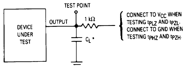
Figure 4. Test Circuit
