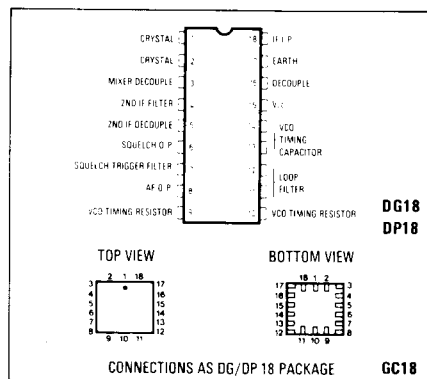
Fig. 1 Pin connections
