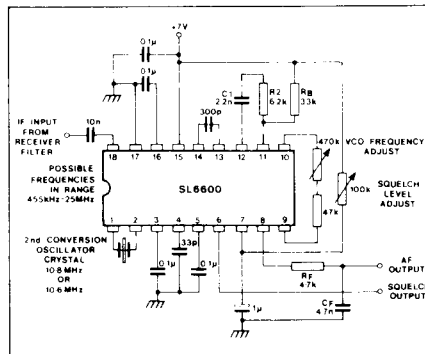
Fig. 3 SL6600 application diagram (1st IF = 10.7 MHz, 2nd IF = 100 kHz)
