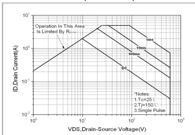
Fig.7. Maximum safe operating area(TO-220FT)
