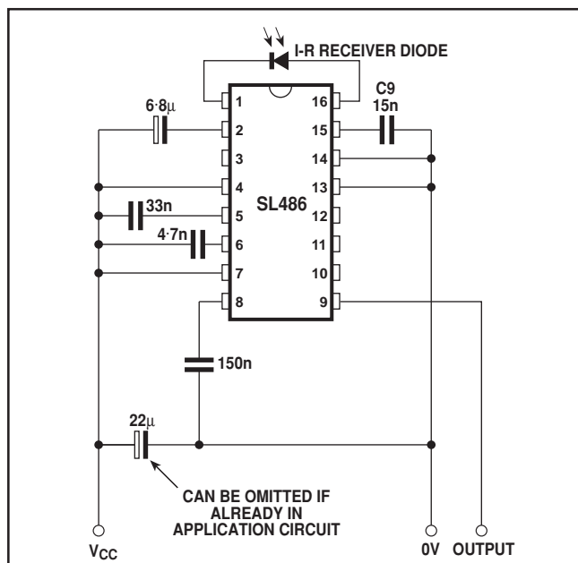
Fig. 3 Circuit diagram of minimum component application (low voltage operation)
