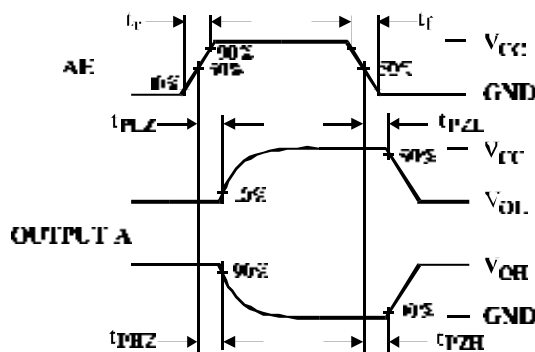
Figure 3. Switching Waveforms
