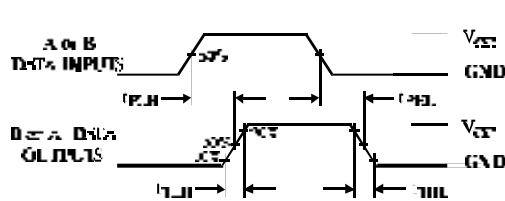
Figure 1. Asynchronous operation
