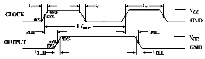
Figure 2. Synchronous operation
