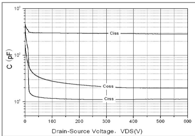
Fig.13. Capacitance characteristics
