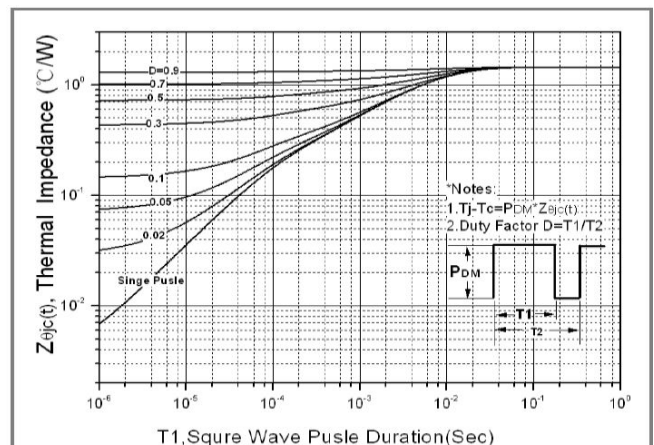
Fig.12. Transient thermal response curve(DPAK)
