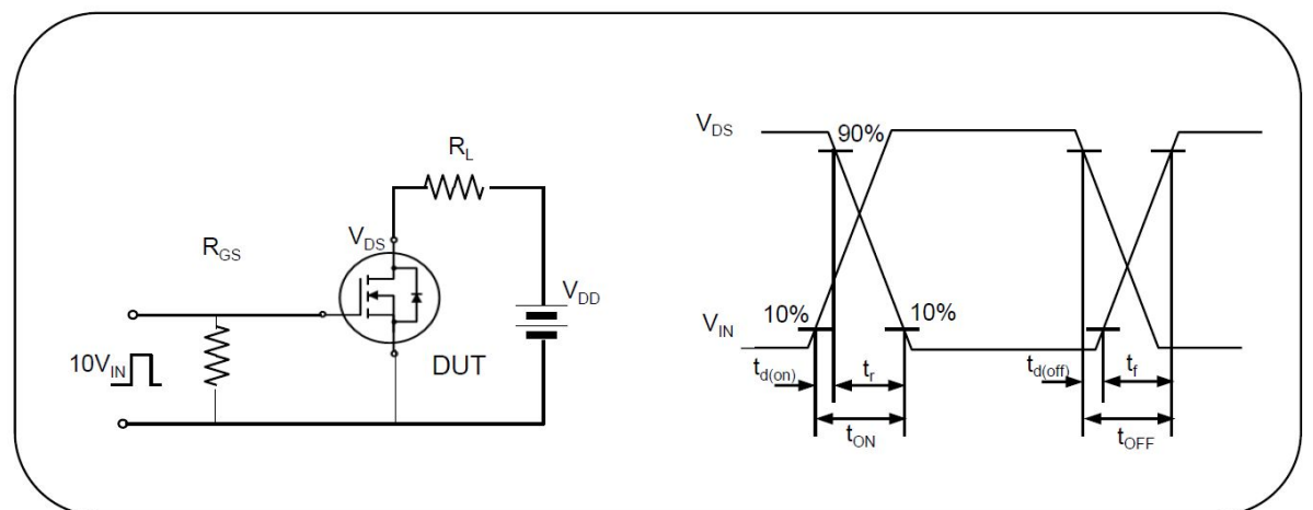
Fig.15. Switching time test circuit & waveform
