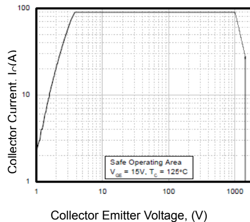
Figure 16. Turn-Off SOA
