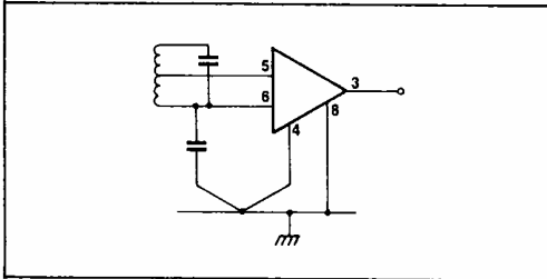
Fig. 4 Alternative input circuit
