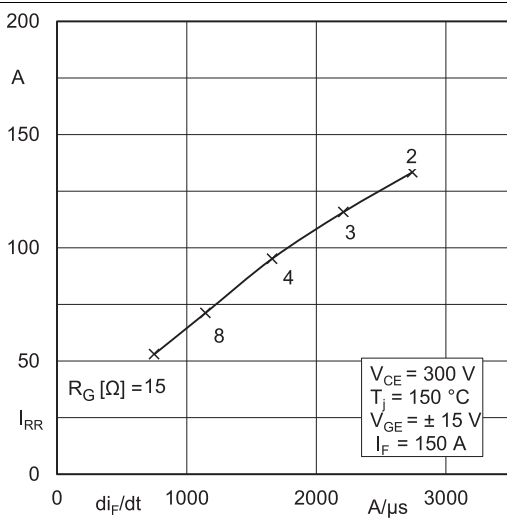
Fig. 11: Typ. Diode5 peak reverse recovery current
