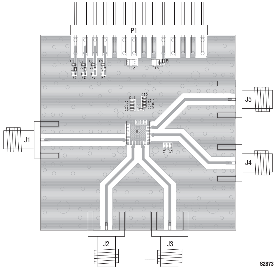
Figure 20. SKY65364-11 Evaluation Board Assembly Diagram
