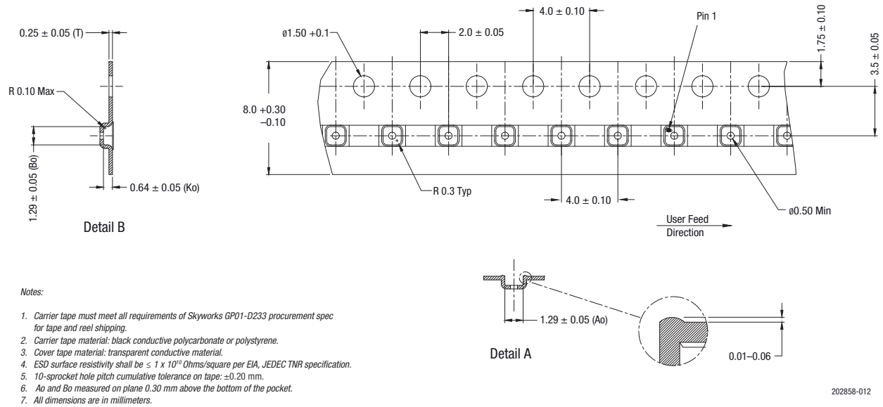
Figure 12. SKY13522-644LF Tape and Reel Dimensions
