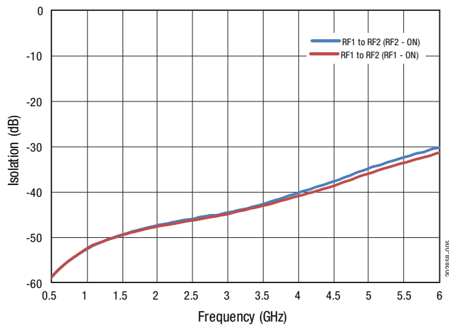
Figure 5. Typical Isolation
