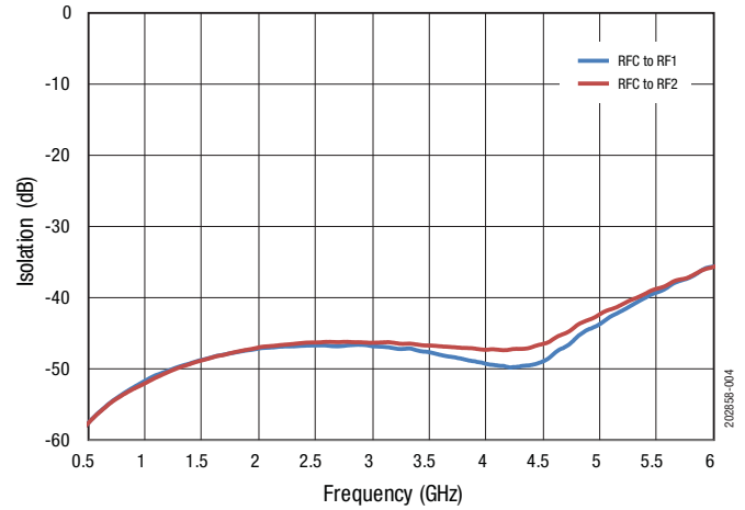
Figure 4. Typical Isolation
