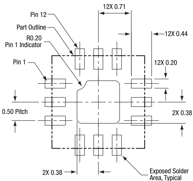
Figure 11. SKY13388-465LF PCB Layout Footprint (Top View)
