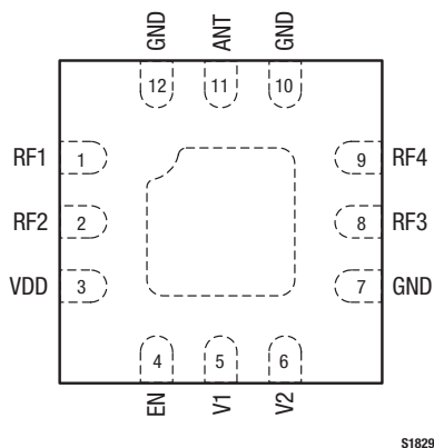
Figure 2. SKY13388-465LF Pinout (Top View)
