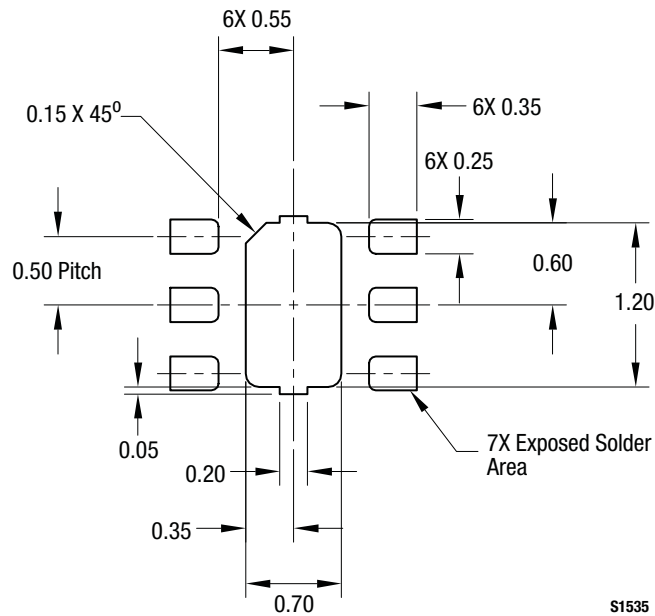
Figure 9. SKY13370-374LF PCB Layout Footprint (Top View)
