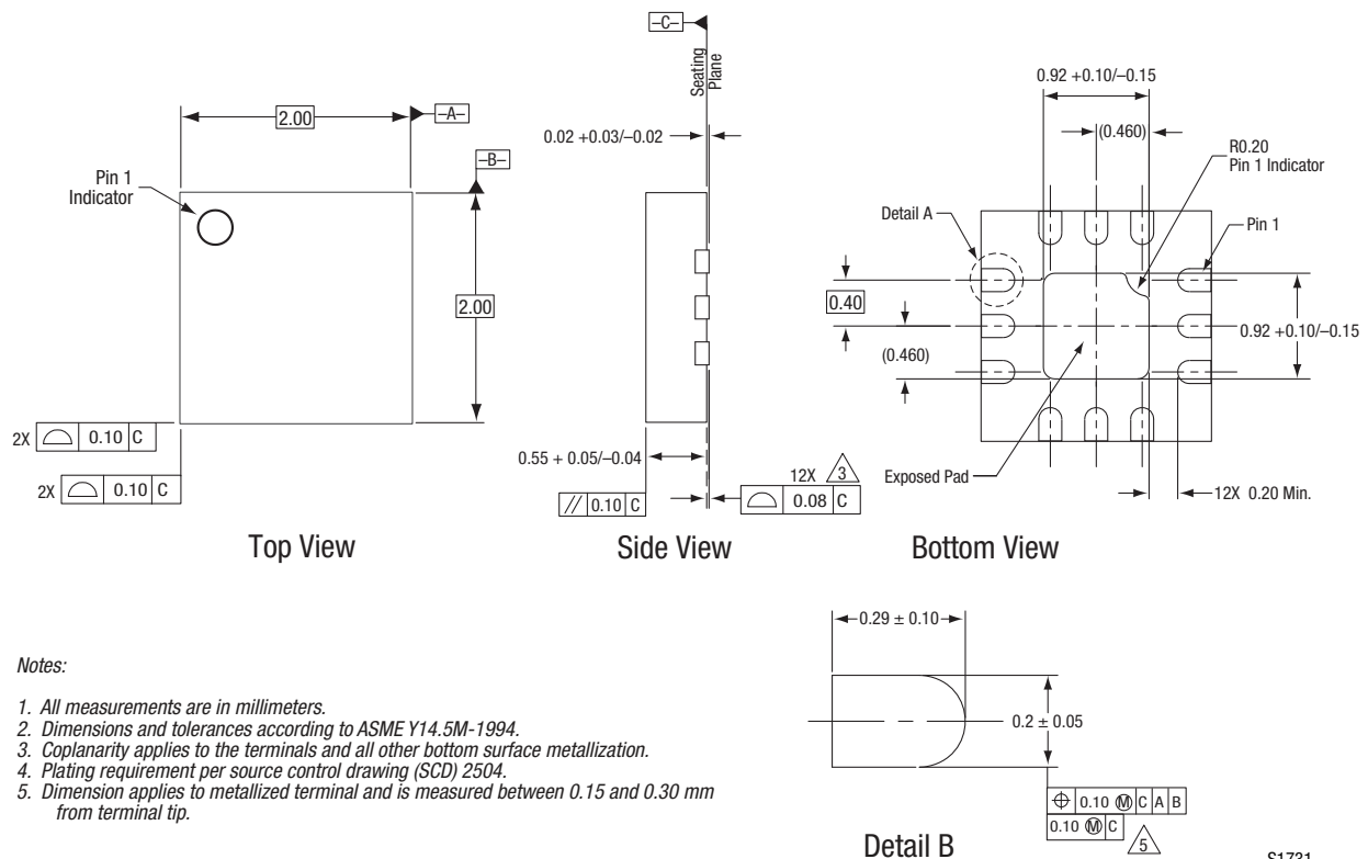
Figure 12. SKY13345-368LF 12-Pin QFN Package Dimensions
