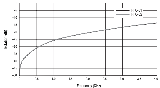
Figure 4. Typical Isolation
