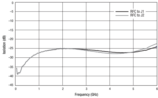
Figure 4. Typical Isolation
