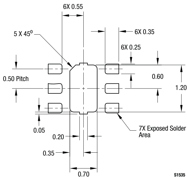
Figure 8. SKY13320-374LF PCB Layout Footprint (Top View)
