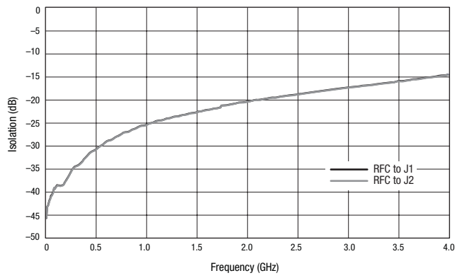
Figure 4. Typical Isolation
