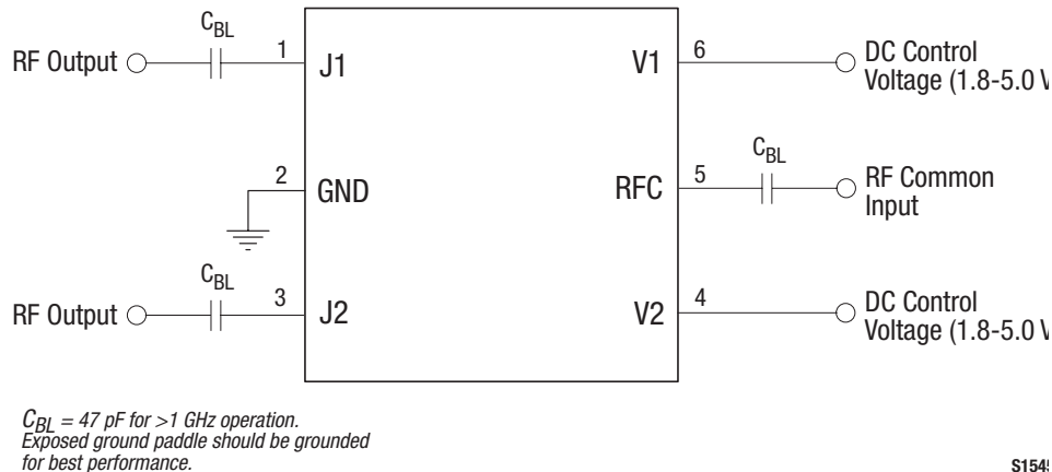
Figure 6. SKY13319-374LF Evaluation Board Schematic
