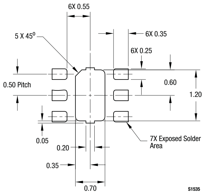
Figure 8. SKY13319-374LF PCB Layout Footprint (Top View)
