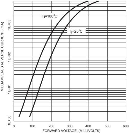
FIG.6- TYPICAL FORWARD CHARACTERISTICS (FOR SKLL22A)
