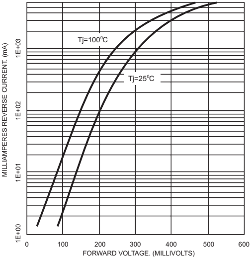
FIG.8- TYPICAL FORWARD CHARACTERISTICS (FOR SKLL24A)
