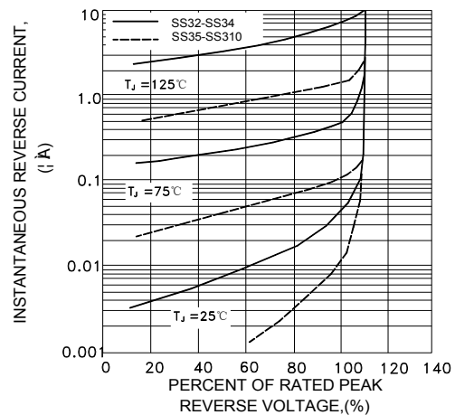
FIG.4-TYPICAL REVERSE CHARACTERISTICS
