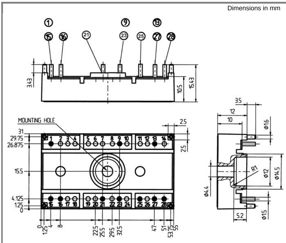
Case T39 (Suggested hole diameter in the PCB for mounting plastic pins and for solder pins= 2mm)
