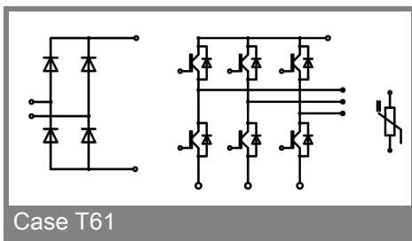
Case T 61 (Suggested hole diameter, in the PCB, for solder pins and plastic mounting pins: 2mm)
