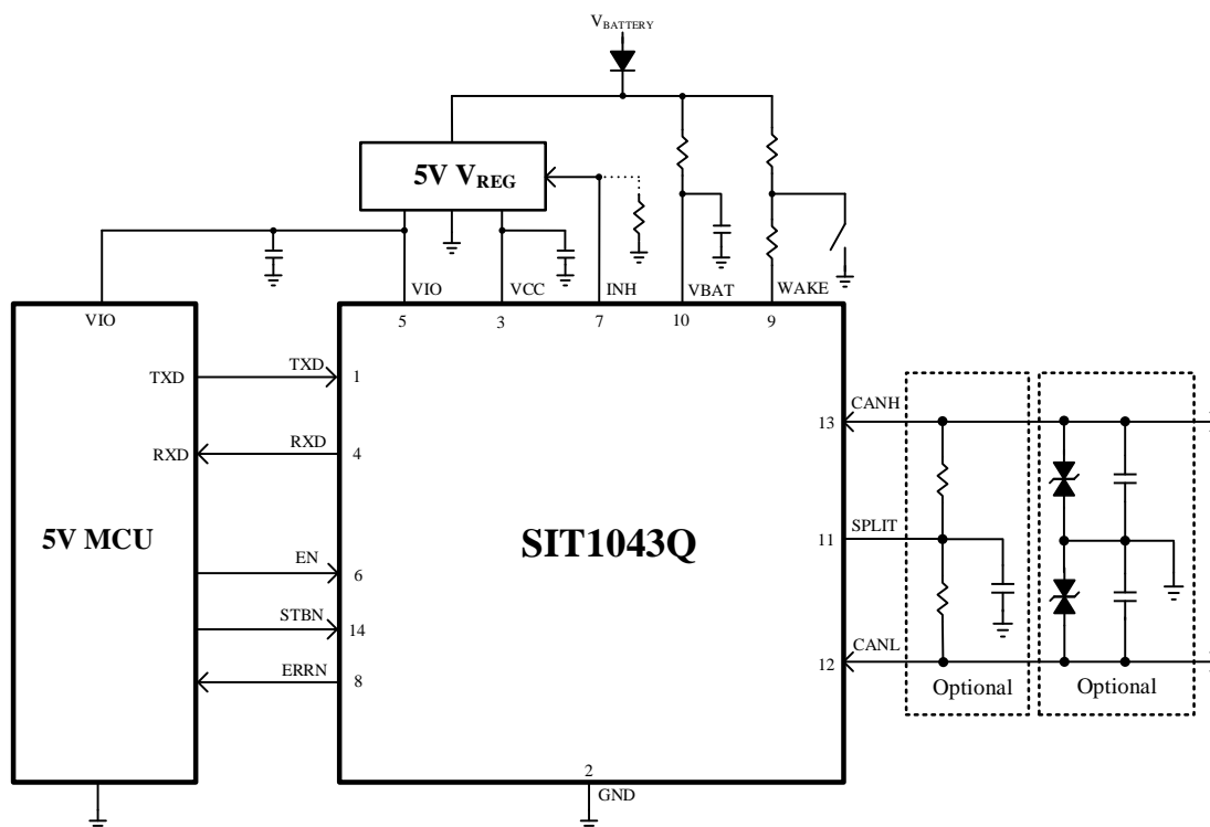
Fig 12 Typical application with 5V MCU
