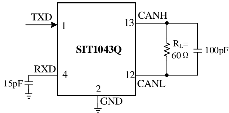
Fig 10 Transceiver timing sequence test circuit
